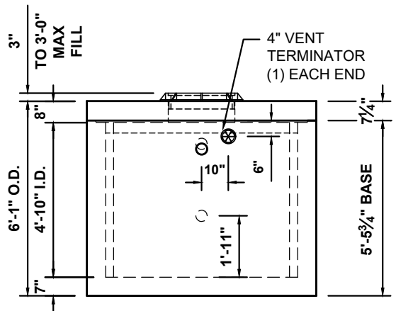
VIEW-B
